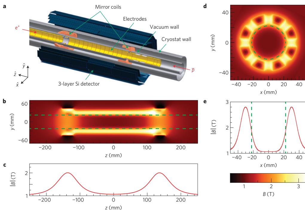
Figure 1 | The ALPHA antihydrogen trap and its magnetic-field configuration. a , A schematic view of the ALPHA trap. Radial and axial confinement of antihydrogen atoms is provided by an octupole magnet (not shown) and mirror magnets, respectively. Penning trap electrodes are held at \sim 9 K, and have an inner diameter of 44.5 mm. A three-layer silicon vertex detector surrounds the magnets and the cryostat. A 1 T base field is provided by an external solenoid (not shown). An antiproton beam is introduced from the right, whereas positrons from an accumulator are brought in from the left. b , The magnetic-field strength in the y - z plane ( z is along the trap axis, with z = 0 at the centre of the magnetic trap). Green dashed lines in this and other figures depict the locations of the inner walls of the electrodes. c , The axial field profile, with an effective trap length of \sim 270 mm. d , The field strength in the x - y plane. e , The field-strength profile along the x axis.
