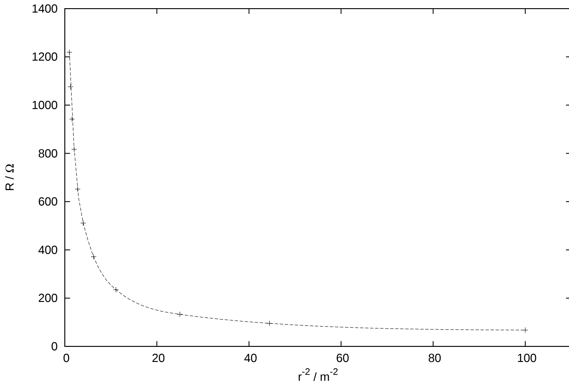
Dependence of LDR resistance on light intensity
